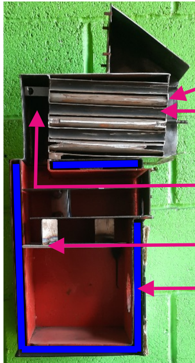
HEAT EXCHANGER CUT-AWAY
